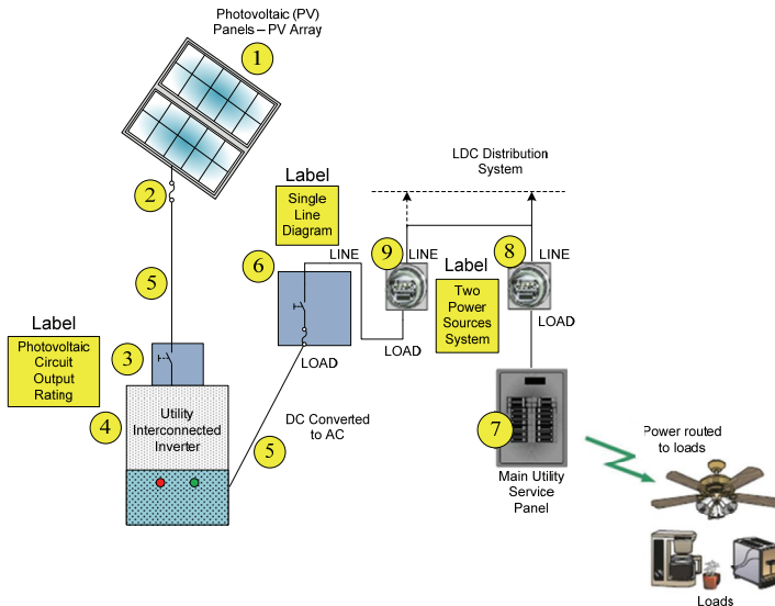
Diagram A: Parallel Meter Connection – microFIT Project
